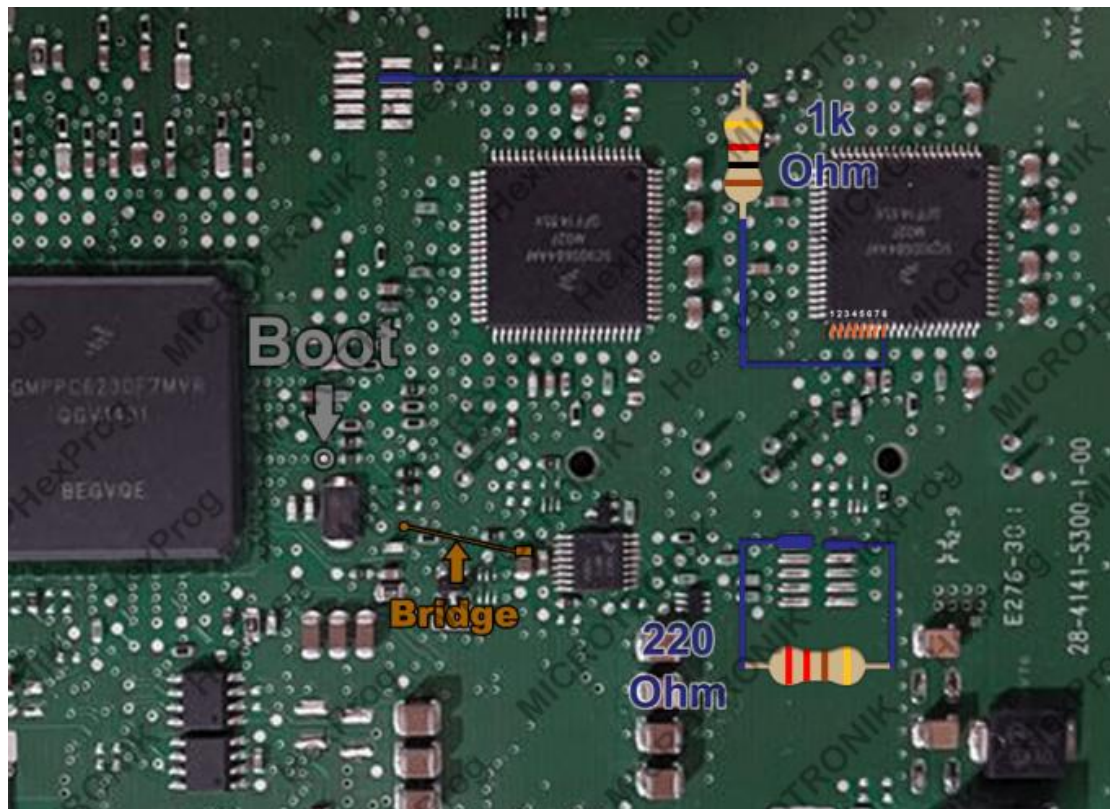
Holden-E39A-Boot-Location
